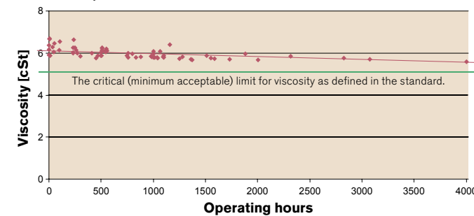
Shear stability of Volvo Automatic Transmission Fluid AT102, Viscosity at 100°C
